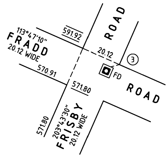
ENLARGEMENT A2 NOT TO SCALE
